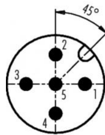
Stecker male
