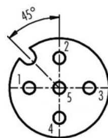
Buchse female
